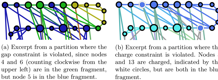
Fig. 1: Examples of violated gap and charge constraints, with fragments represented by colors.
